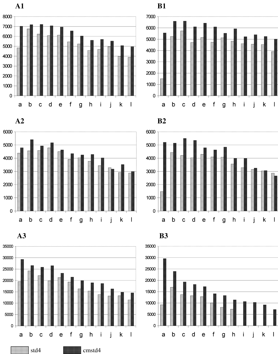
Fig. 6. Long-term stability of responses (peak areas) of (A) heptachlor and (B) dimethoate at 0.05 µg/ml in solvent standards (std4 n ) and matrix-matched standards (cmstd4 n ) for the 12 sets ( n = a-l ) using (1) conventional GC-MS technique, 1 µl injection, (2) LP-GC-MS technique, 1 µl injection, and (3) LP-GC-MS technique, 2 µl injection. See Section 2.3 for a description of the stability study.
